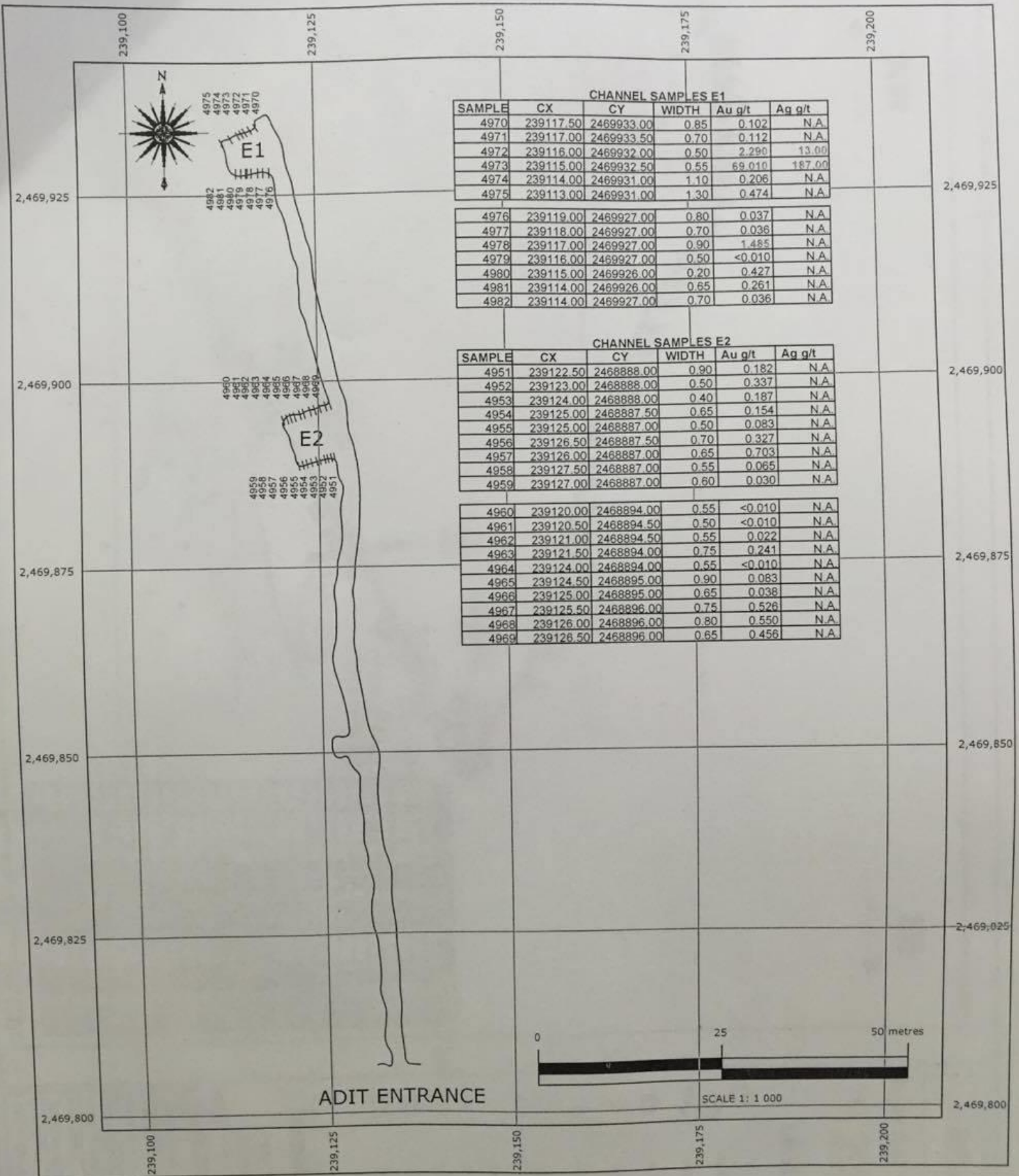
FIGURE 25. CHANNEL SAMPLES FROM THE UNDERGROUND DRILL-HOLE EXCAVATION PADS
